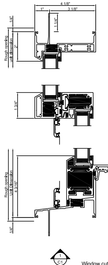
Window cut sections 1 : 4
